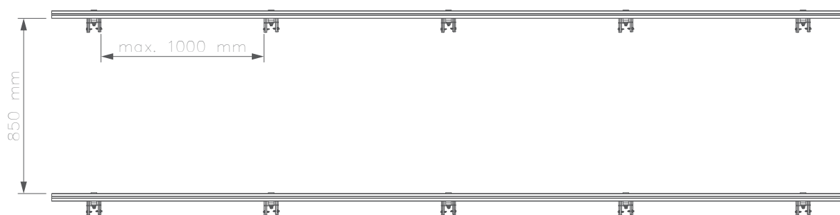
Fig. 2. arrangement of the mounting rails with roof attachment
