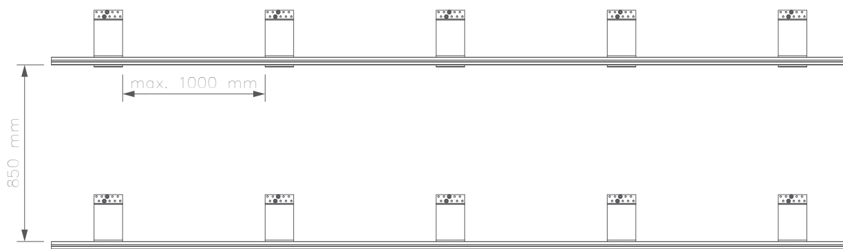
Fig. 2. arrangement of the mounting rails with roof attachment
